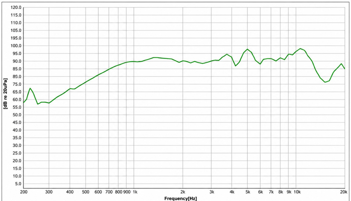
Frequency Response Curve / 频率响应曲线。
