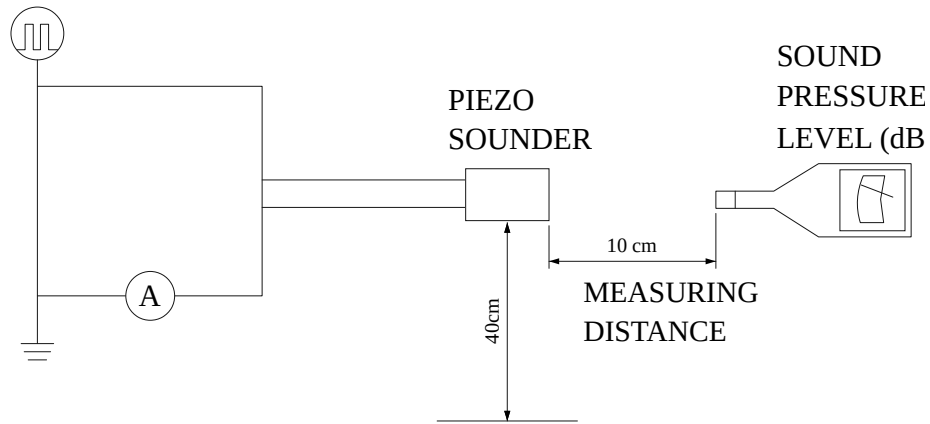
/ Buzzer placement during measurement
