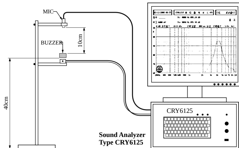
/ Buzzer placement during measurement
