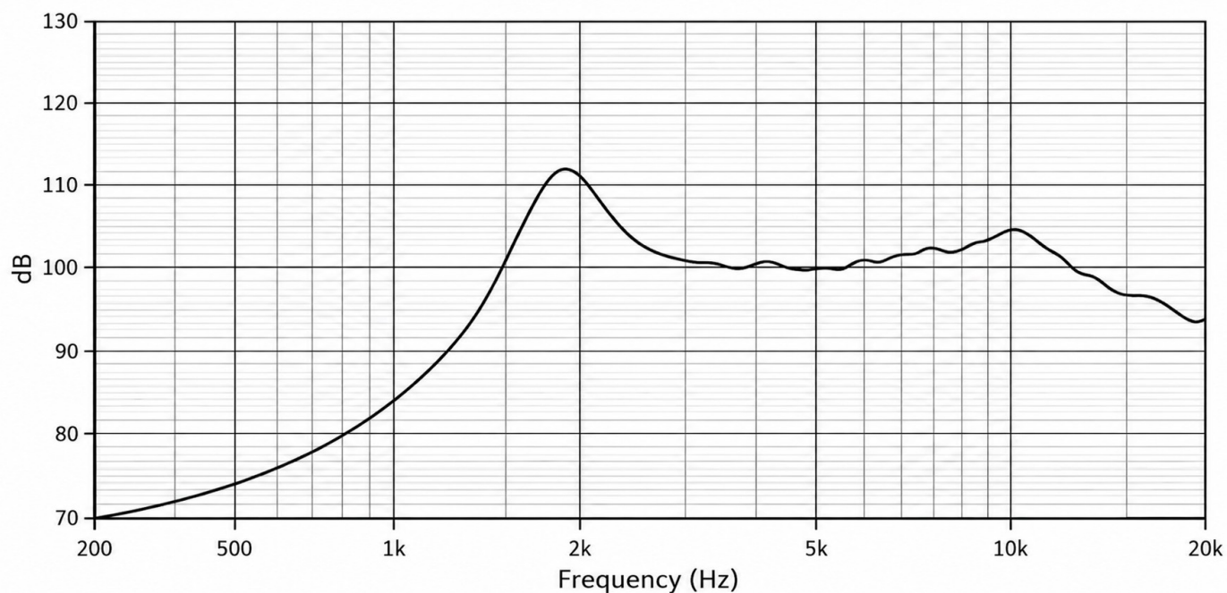
Frequency Response / 频率响应
